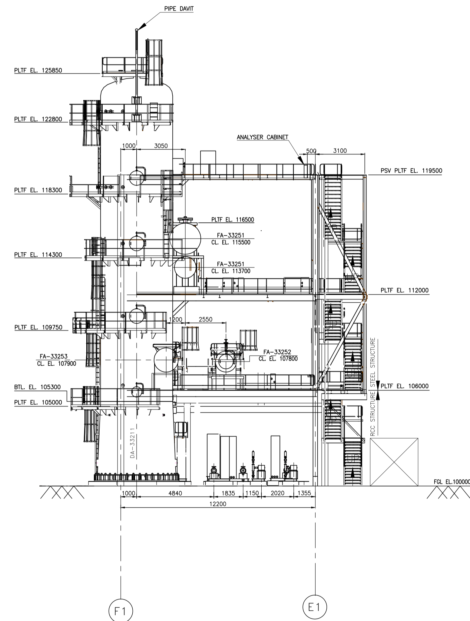
SECTION X-X
