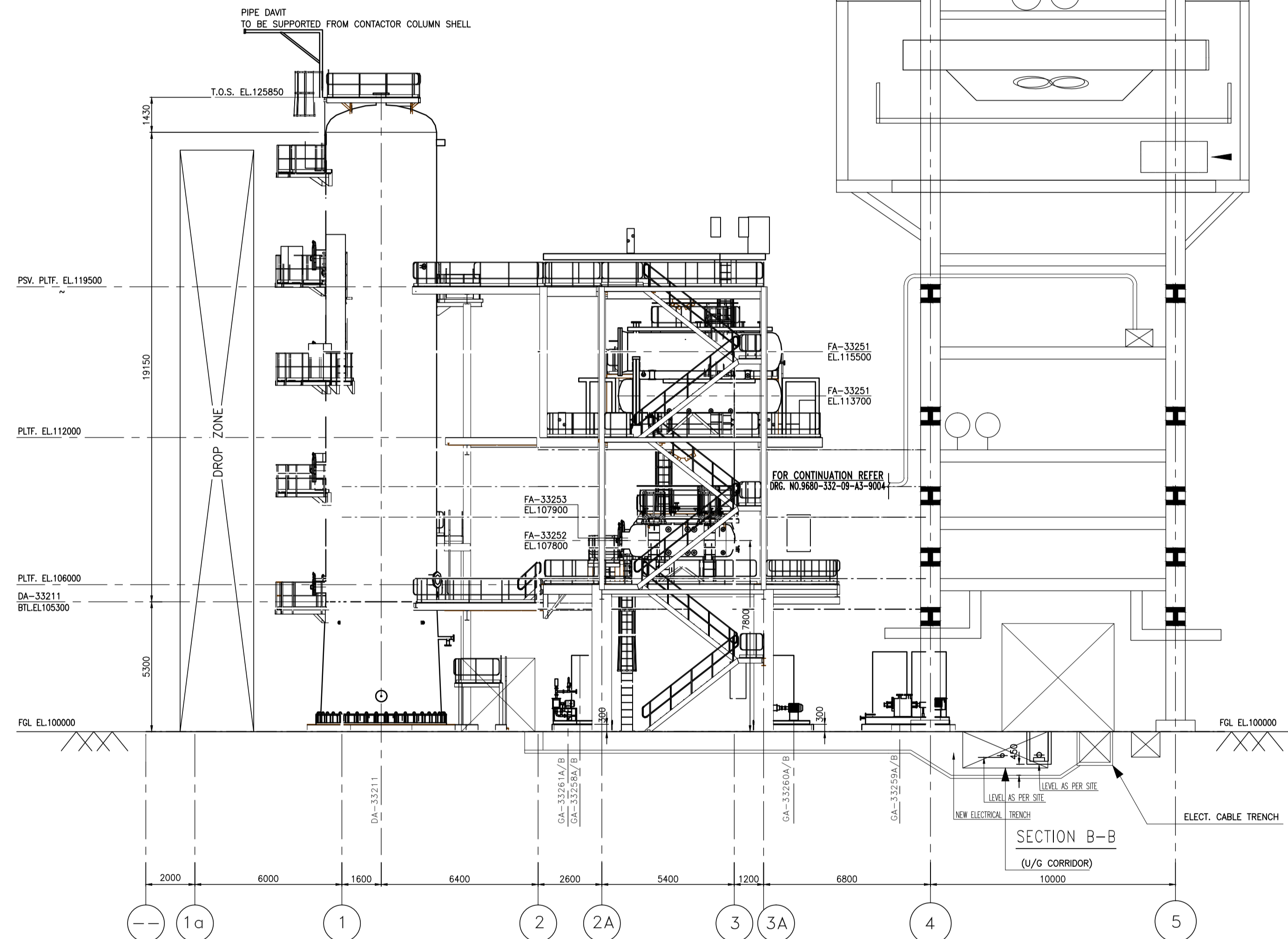
SECTION Y-Y
