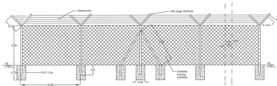
Chain-link Fencing of 2 Meter Height
